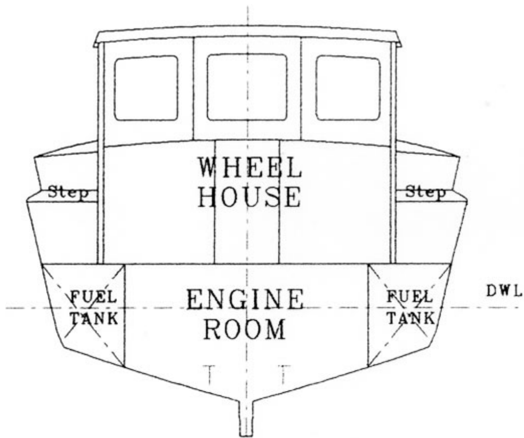
Section at Amidships looking Fwd
